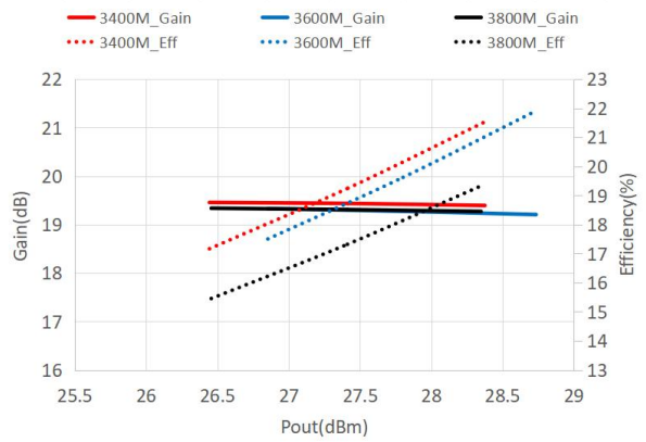
WCDMA performance(Gain+Eff)
