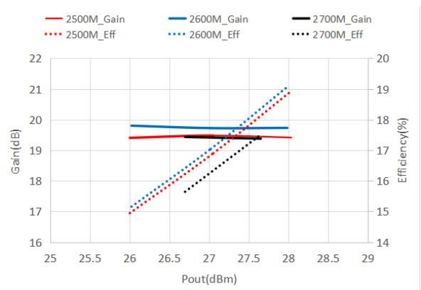
WCDMA performance(Gain+Eff)
